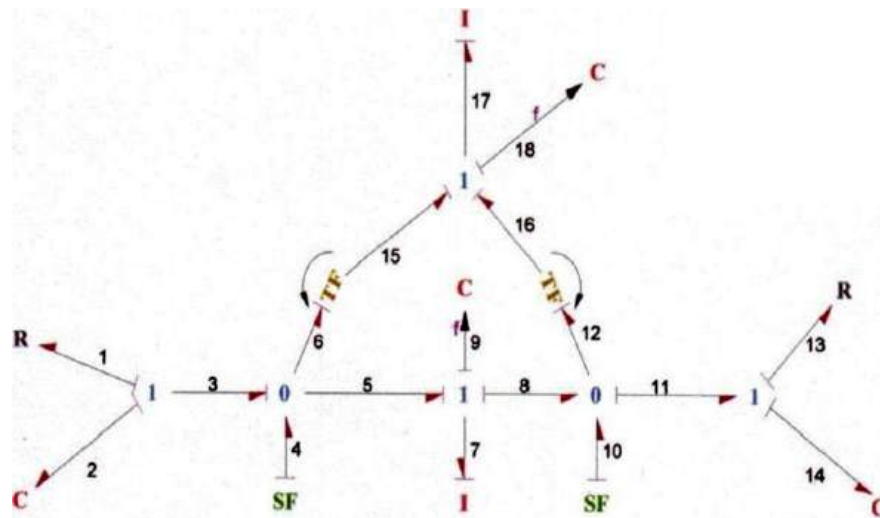
Fig. 4.2 Bond graph model of full car model with a fixed suspension
