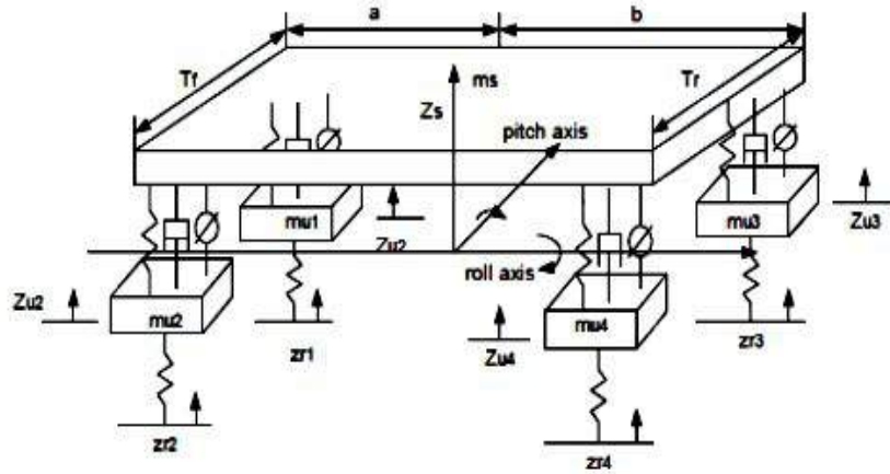
Fig.6.11: Vehicle Representation
