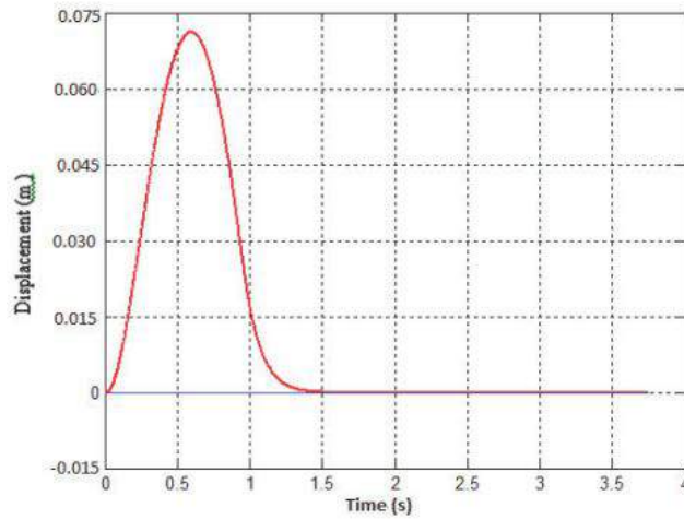
Fig. 6.30: Sprung-mass displacement vs. Time lag for comfort zone, when front tyre damping coefficient , (b_f) = 16 \text{ kNs/m} and speed = 100 km/h.
