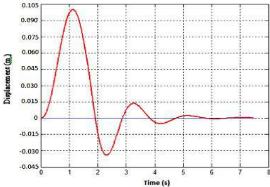
Fig. 6.13: Sprung-mass displacement vs. Time lag for comfort zone, when rear tyre damping coefficient ( b_r ) = 4 kNs/m and speed = 50 km/h
