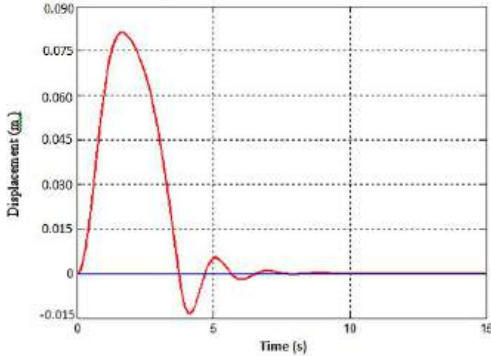
Fig. 6.12: Sprung-mass displacement vs. Time lag for comfort zone, when rear tyre damping coefficient ( b_r ) = 4 kNs/m and speed = 25 km/h.
