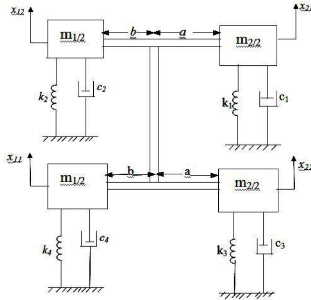
Fig.6.2: Dynamic model with pitching
