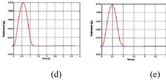
Fig 6.5: Sprung-Mass Displacement vs. Time at Bump height 0.075 m and a speed of (a) 25 km/h, (b) 50 km/h, (c) 75 km/h, (d) 100 km/h, and (e) 125 km/h.
