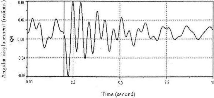
Fig. 4.3: Rocking motion of the full car model at front suspension with vertical angular displacement at C.G., Input parameters to Symbol Shakti, Angular displacement-(Q4 radians), Speed 15 m/s, Time 10 seconds
