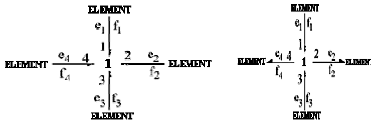
Fig.3.1 '1' Junction Element Models
