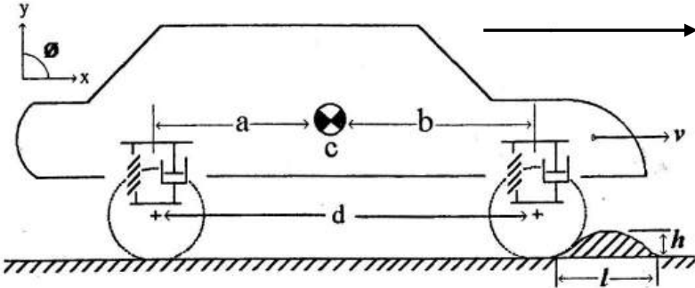
Fig. 4.1 Full car model with a fixed suspension
