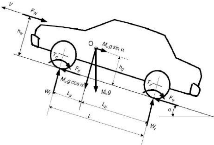
Fig. 2.6 Vehicle longitudinal forces
