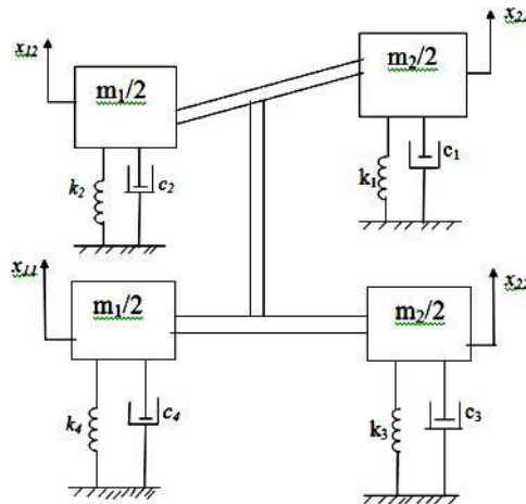
Fig. 6.10: Four wheeled car model having different load
