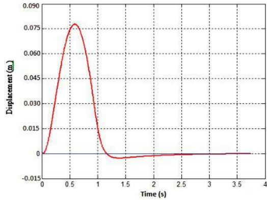
Fig. 6.20: Sprung-mass displacement vs. Time lag for comfort zone, when front tyre damping coefficient ( b_f ) = 8 kNs/m and speed = 100 km/h.
