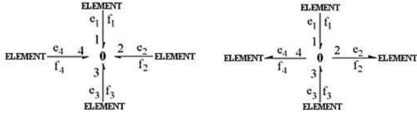
Fig.3.2 '0' Junction Element Models
