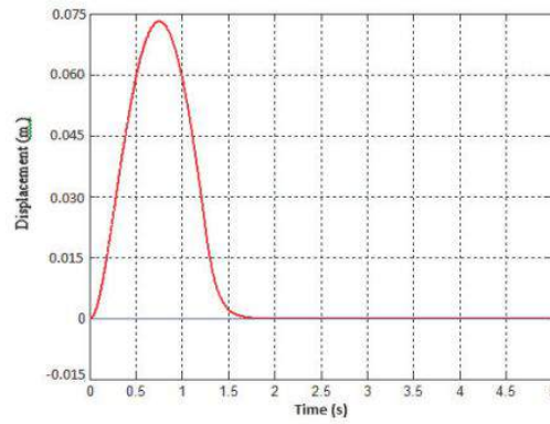
Fig. 6.29: Sprung-mass displacement vs. Time lag for comfort zone, when front tyre damping coefficient , (b_f) = 16 \text{ kNs/m} and speed = 75 km/h.
