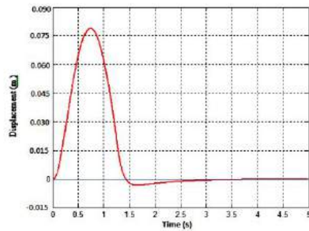
Fig. 6.19: Sprung-mass displacement vs. Time lag for comfort zone, when front tyre damping coefficient ( b_f ) = 8 kNs/m and speed = 75 km/h
