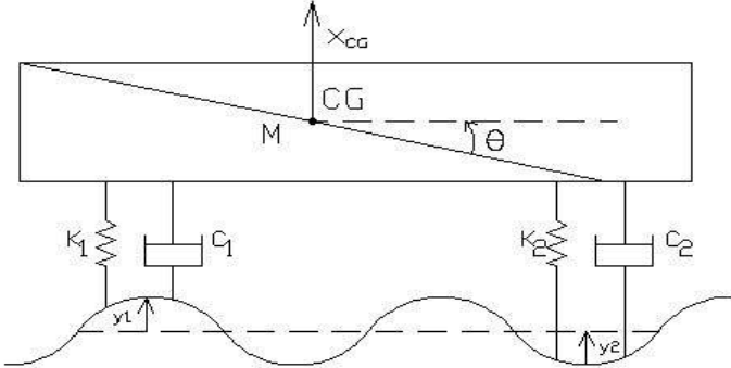
Fig. 2.3 Spring-mass-damper model
