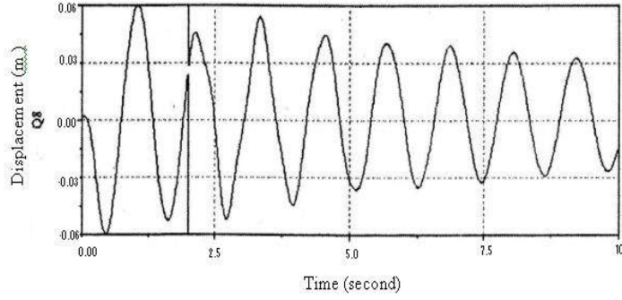
Fig. 4.4: Heaving motion of the full car model at rear suspension with vertical displacement at C.G., Input parameters to Symbol Shakti, Displacement- (Q8 m), Speed 15m/s, Time 10 seconds
