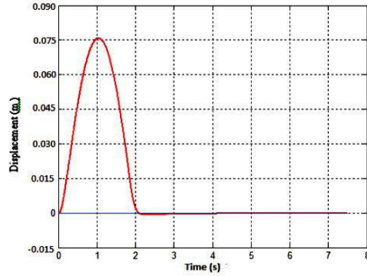
Fig. 6.23: Sprung-mass displacement vs. Time lag for comfort zone, when rear tyre damping coefficient ( b_r ) = 12 kNs/m and speed = 50 km/h.
